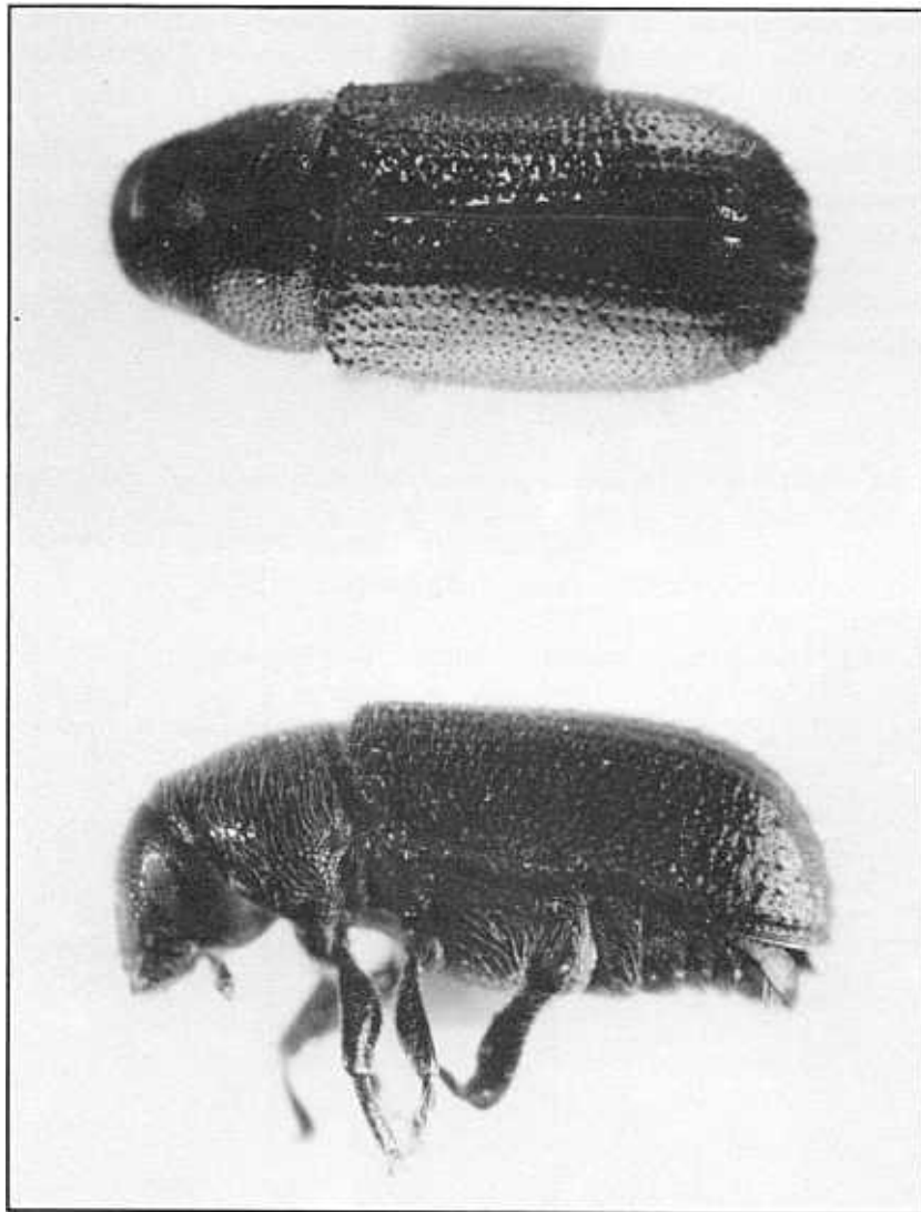
Figures 1-2. Tomicus piniperda (Linnaeus), adult. 1) Dorsal view; 2) lateral view. DPI photo by Jeffrey Lotz.
