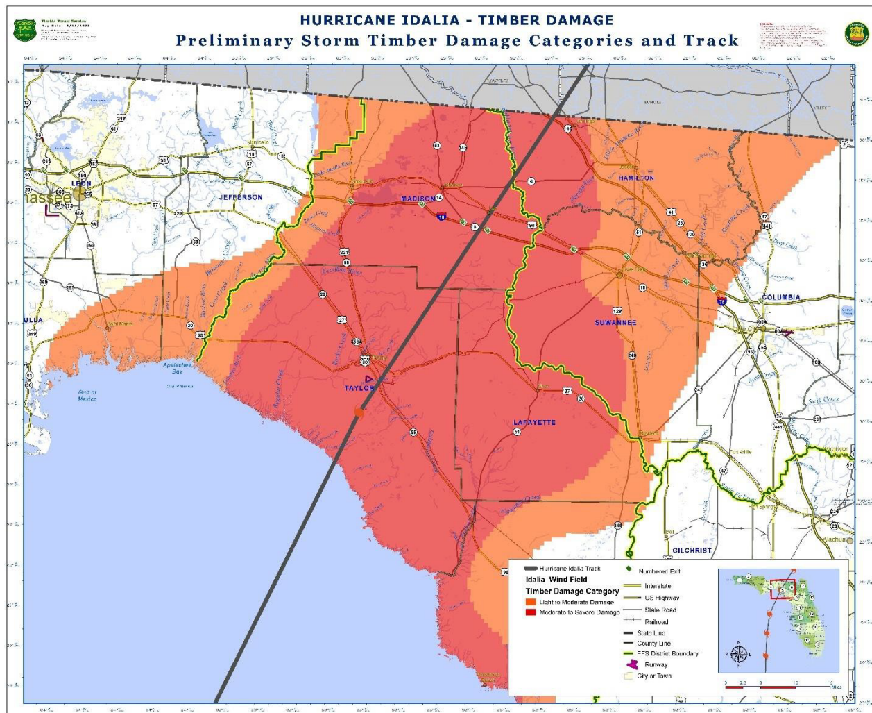
Figure 4 Timber damage maps showing storm track and estimated damage categories based on ground observations and wind speeds.
