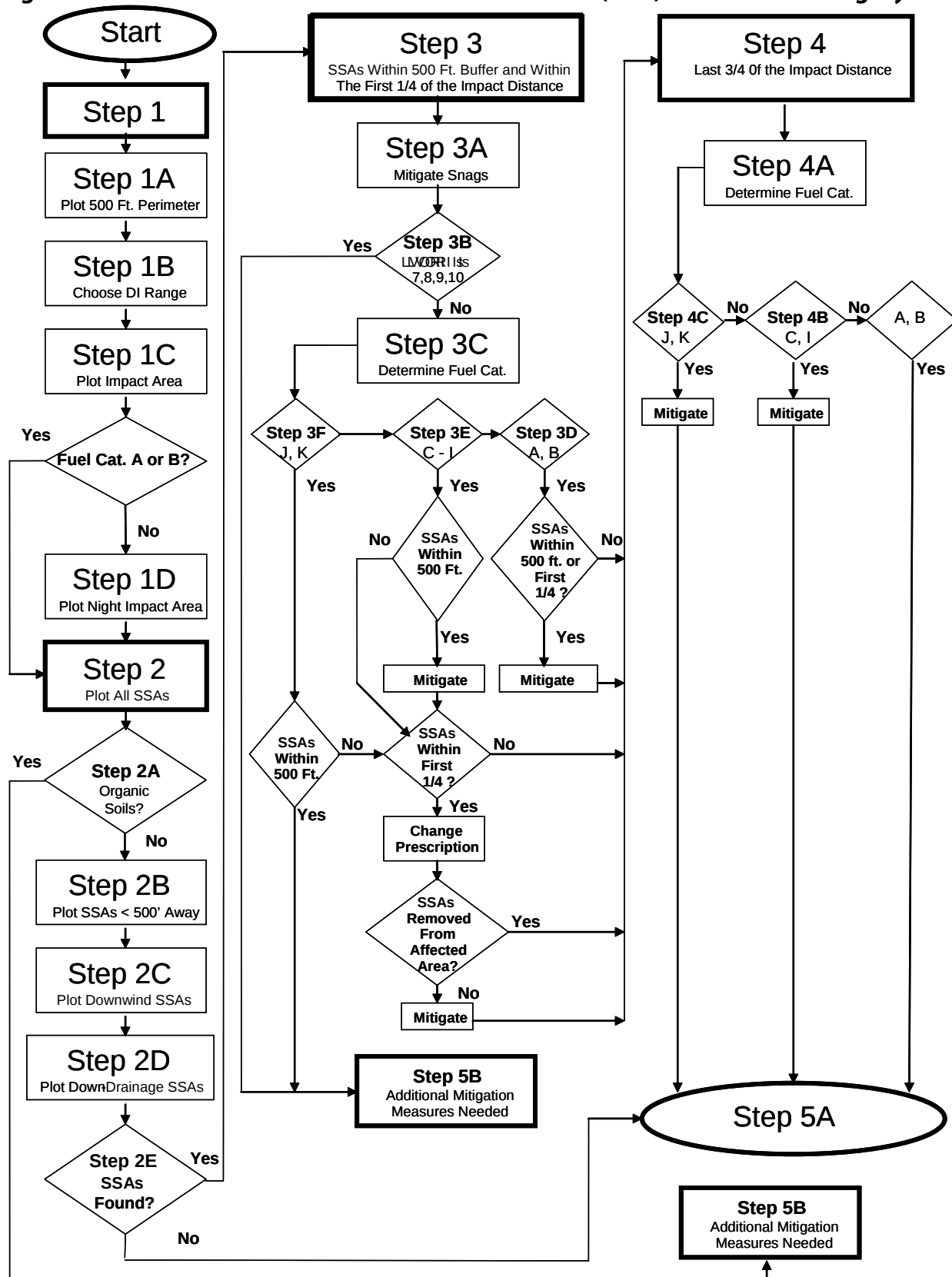
Fig. 2 – Flowchart of the Wildland/Urban Interface (WUI) Smoke Screening System
