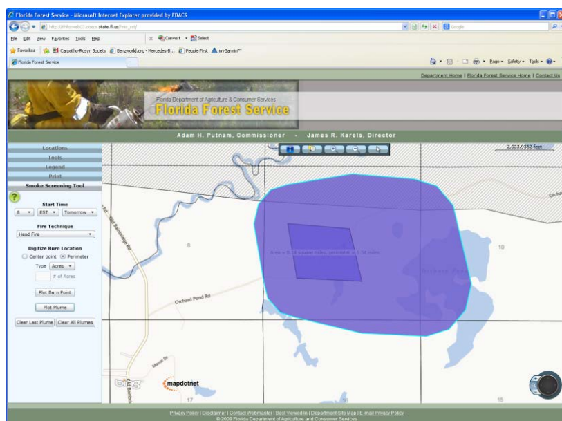
Fig. 1 - Smoke plume surface concentration above 300 \mu\text{g m}^{-3} using FFS Smoke Screening
